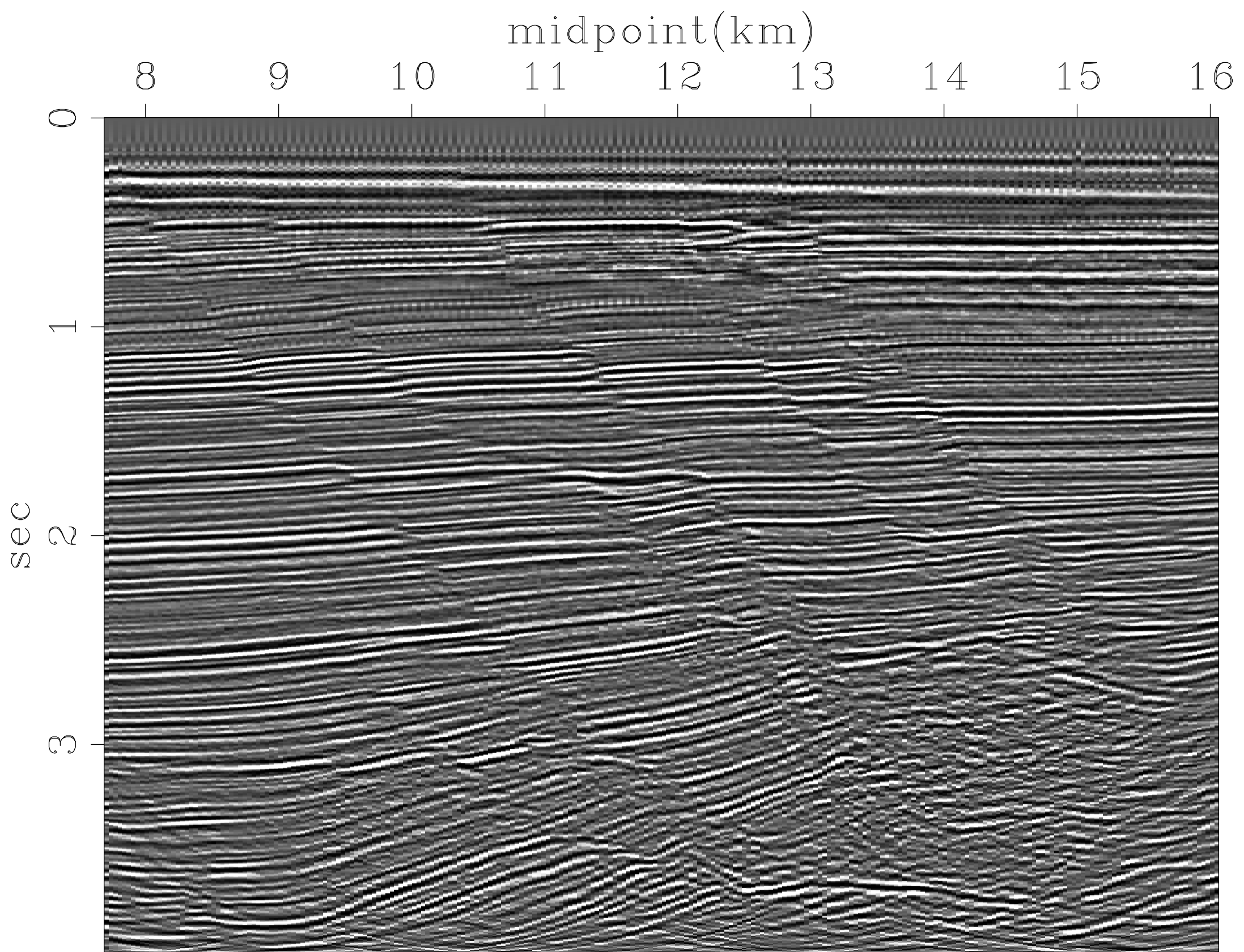
Kirchhoff migration
