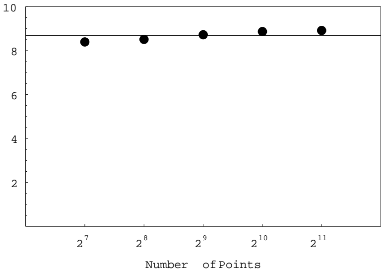
Number of InCircleTests per Point
