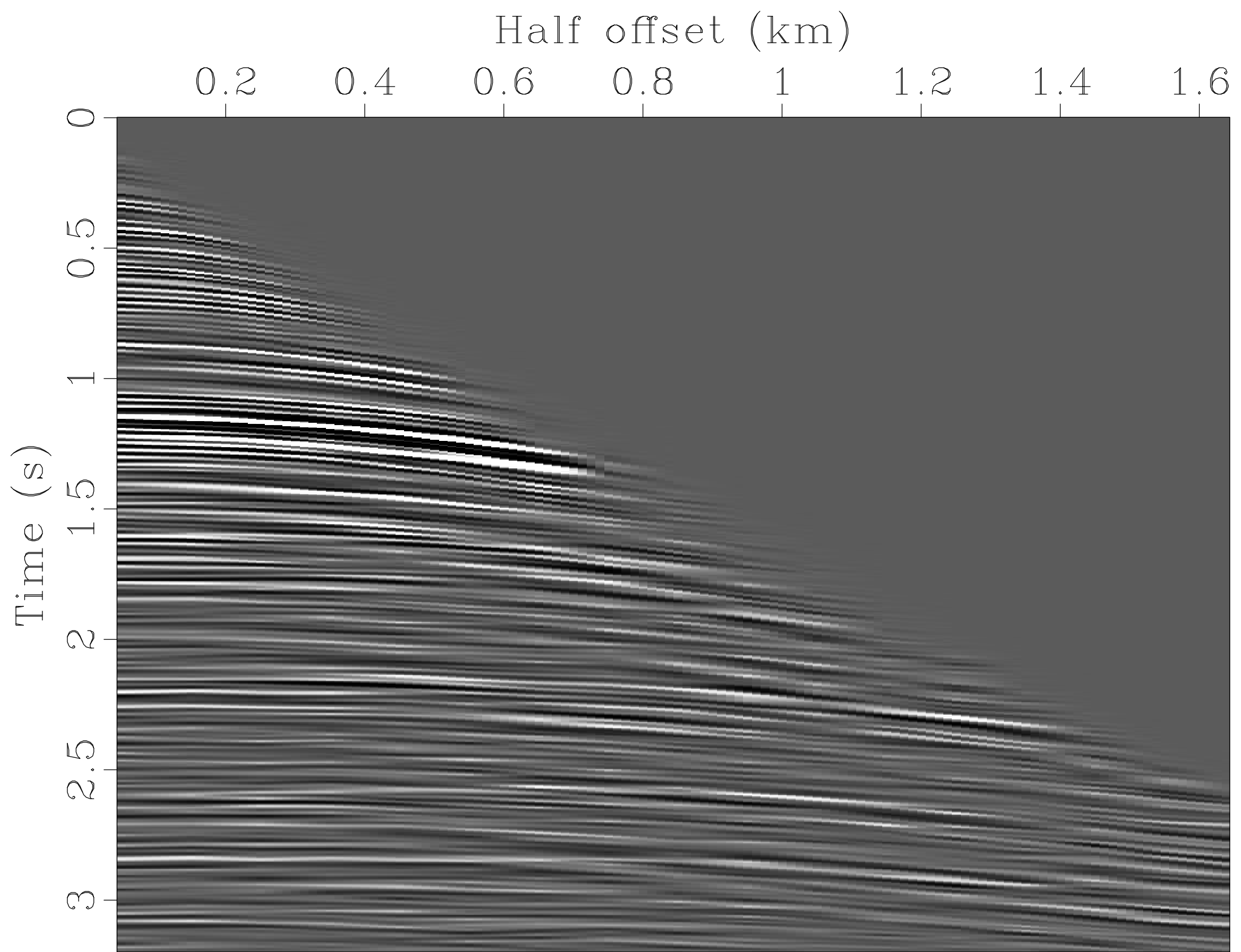
Denoising result
