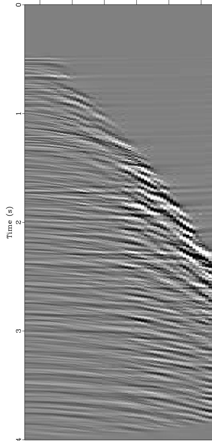
Inverse Hyperbolic Radon Transform
