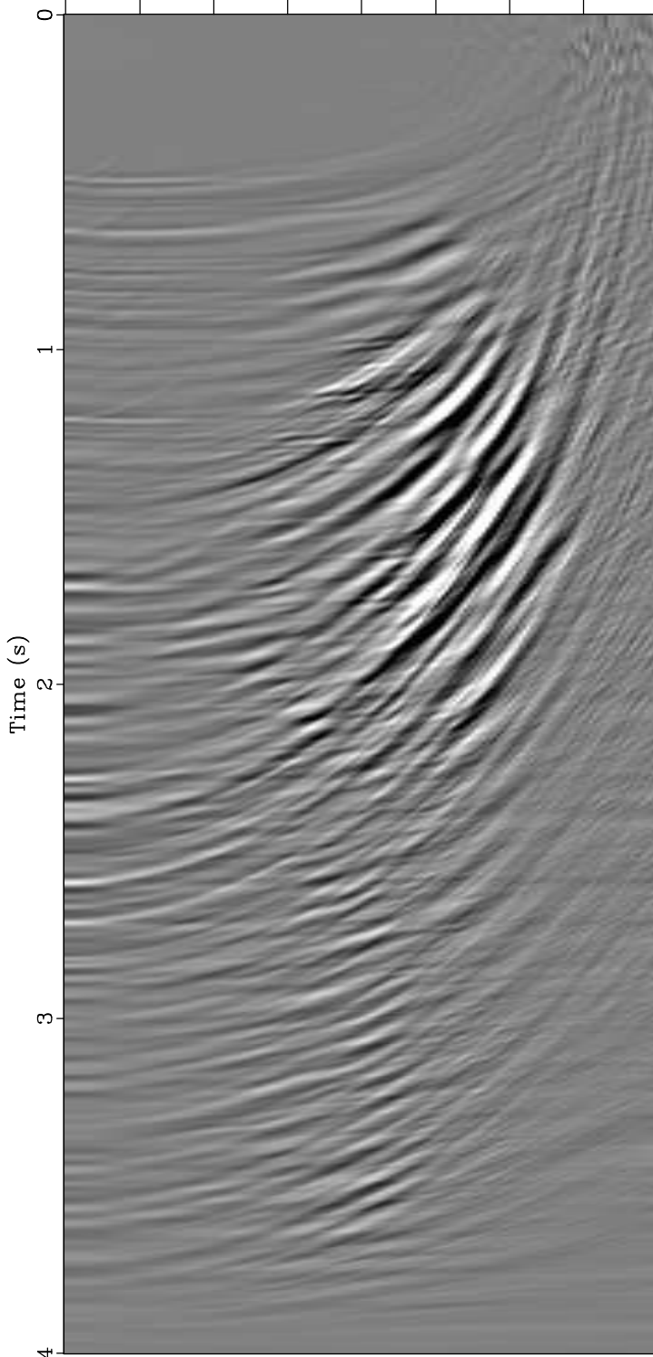
Hyperbolic Radon Transform
