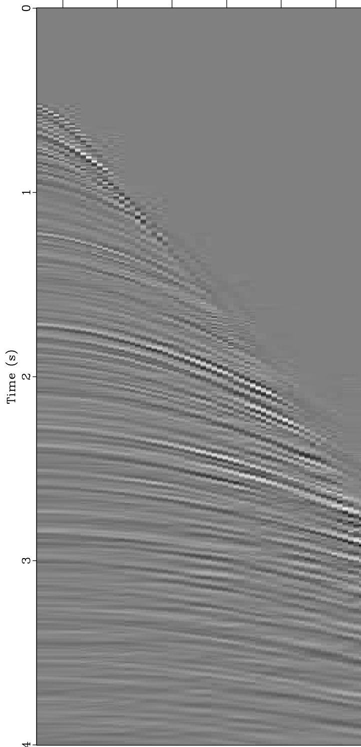
Demultiple
