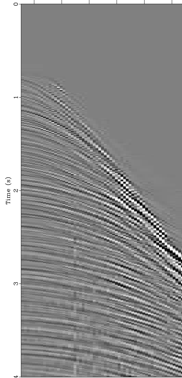
Multiples
