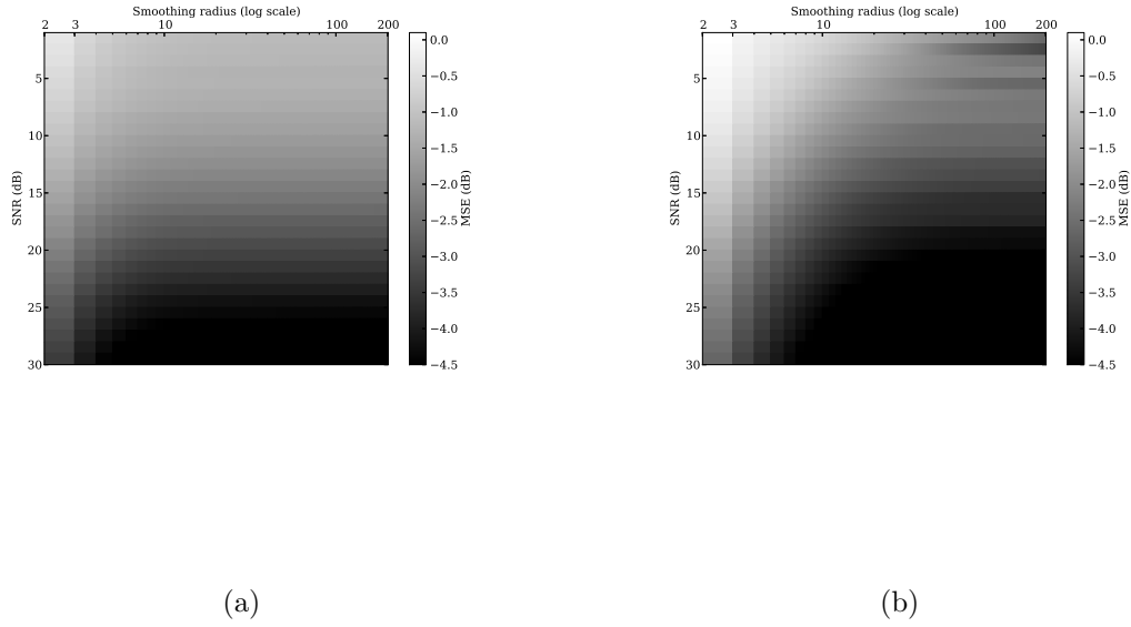
Figure 3: Mean square errors of of the slope estimations by the proposed method (a) and the three-point ( N = 1 ) iterative method (b).
