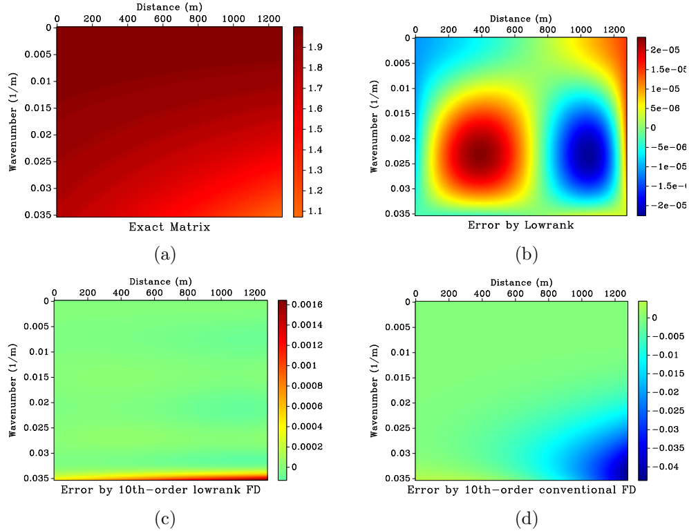
Figure 1: (a) Wavefield extrapolation matrix for 1-D linearly increasing velocity model. Error of wavefield extrapolation matrix by: (b) lowrank approximation, (c) the 10th-order lowrank FD (d) the 10th-order FD.
