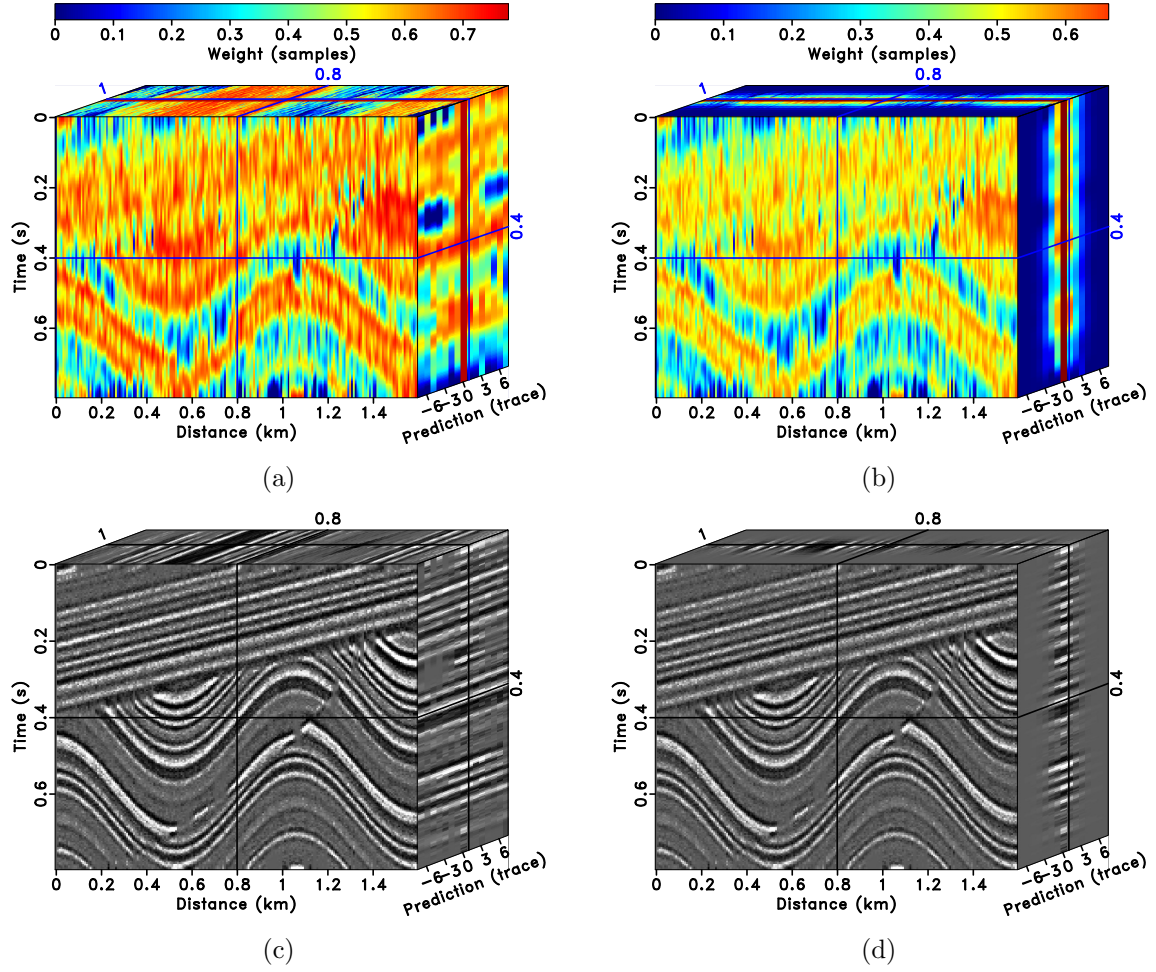
Figure 2: Similarity weights (a), product of Gaussian weights and similarity weights (b), the data only with similarity weights applied (c), and the data with Gaussian similarity weights applied (d).
