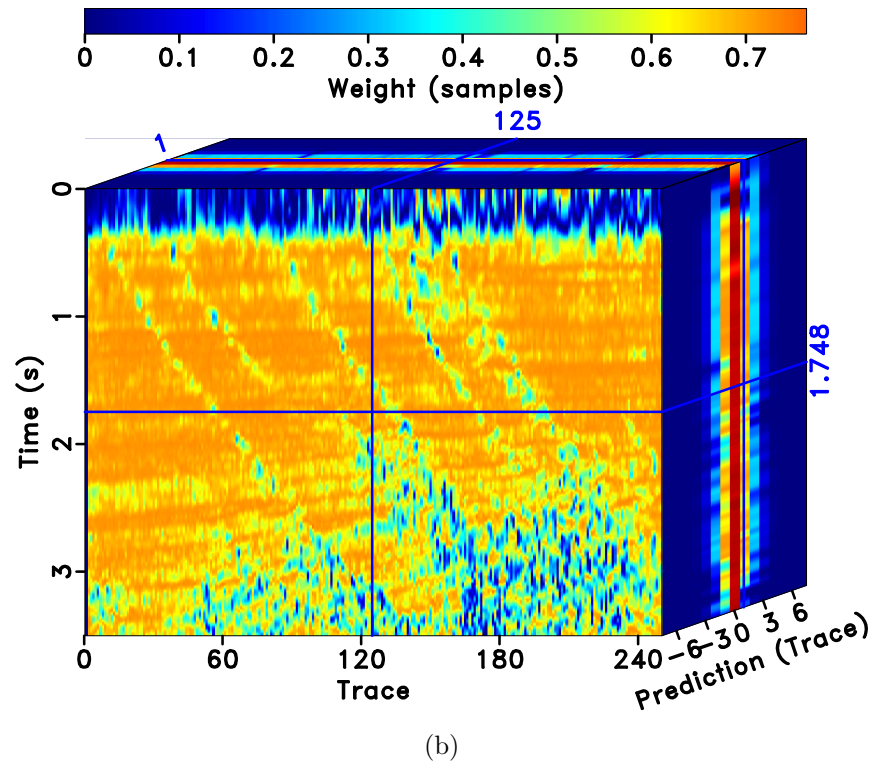
Figure 7: Predictive data volume (a) and product of Gaussian weights and similarity weights (b).
