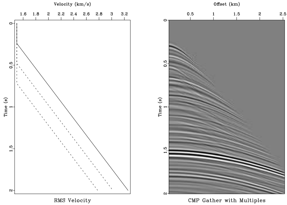
Figure 2: RMS velocity profiles for primaries and multiples (left) and synthetic multiple-infected CMP gather (right). synth/ cmp2
