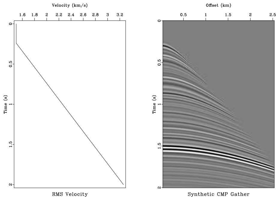
Figure 1: RMS velocity profile (left) and synthetic CMP gather (right). synth/ cmp
