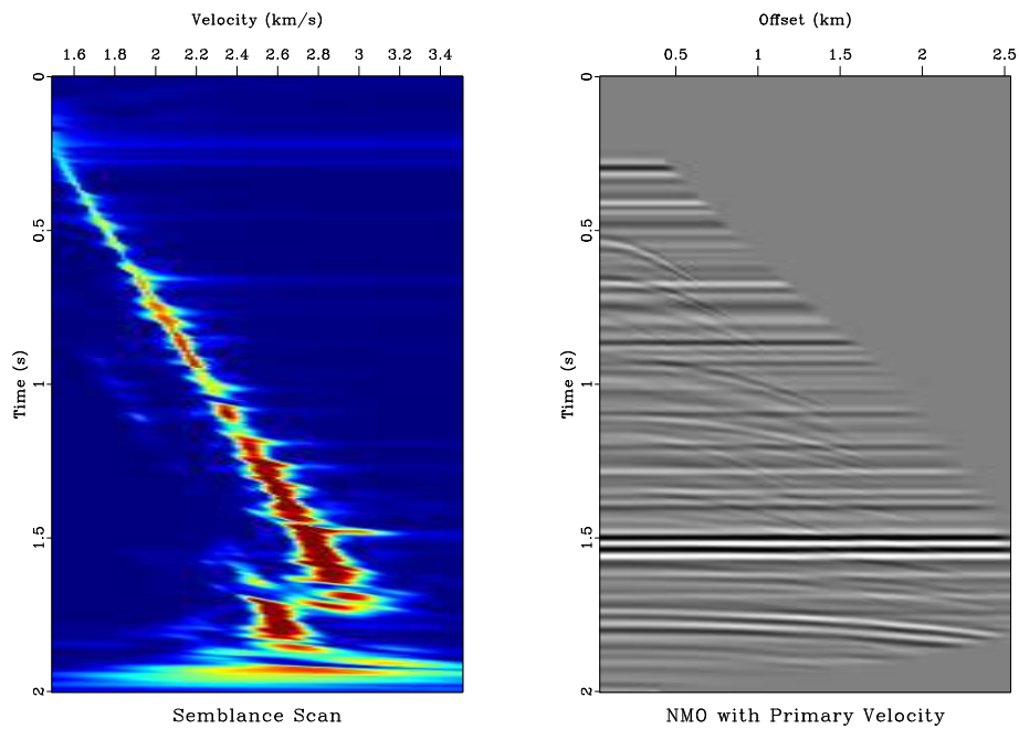
Figure 3: Semblance scan (left) and NMO with the primary velocity (right) applied to the synthetic CMP gather from Figure 2. synth/ nmo
