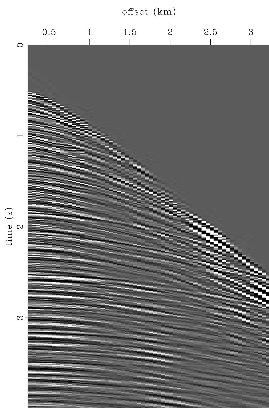
Input CMP gather
