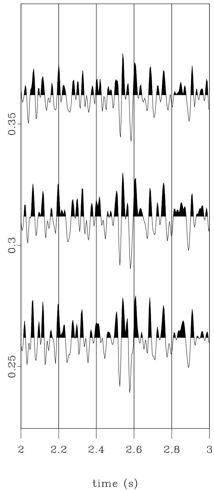
Velocity Stack
