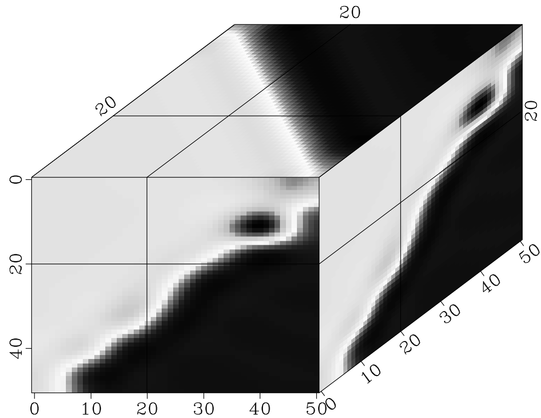
X slope
