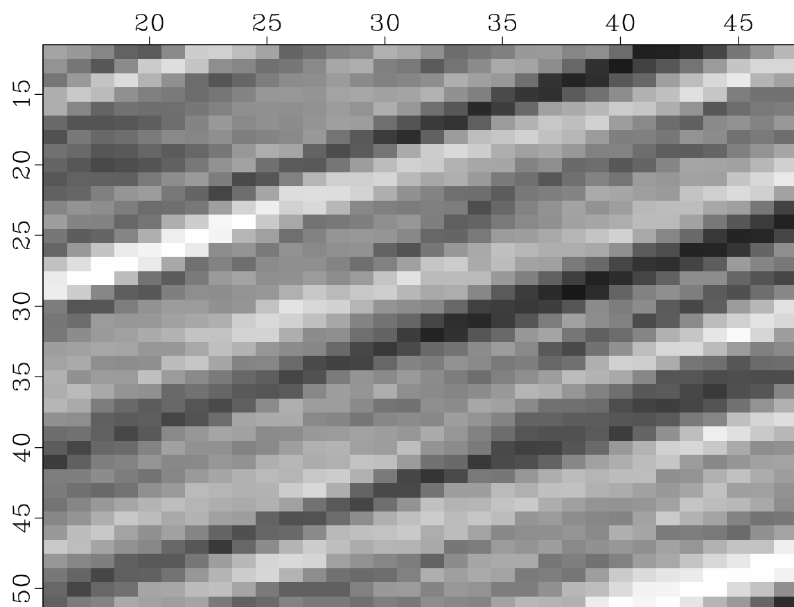
6-point Lagrange
