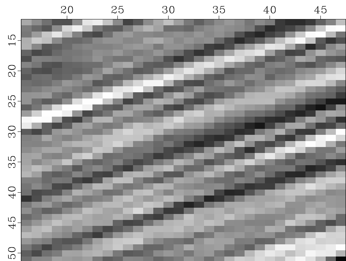
8-point Sinc
