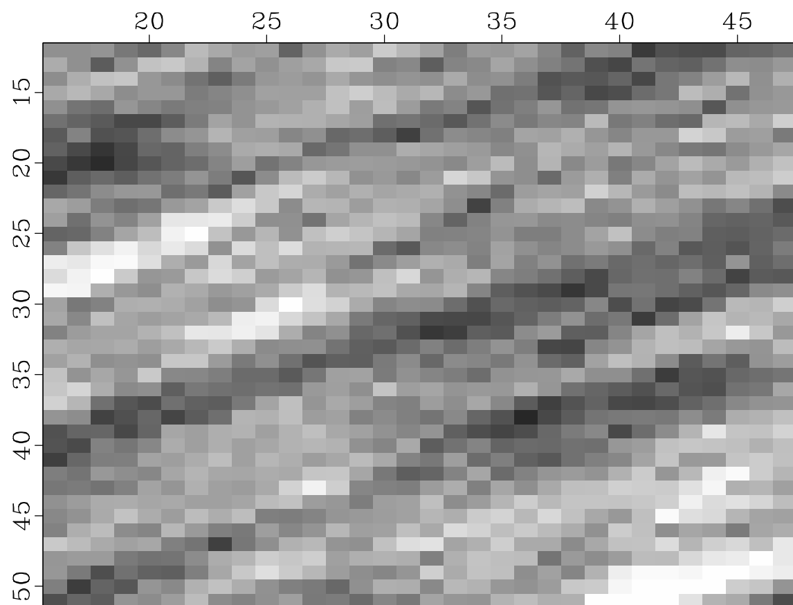
2-point Linear
