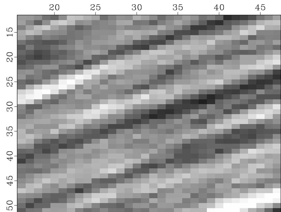
4-point Cubic
