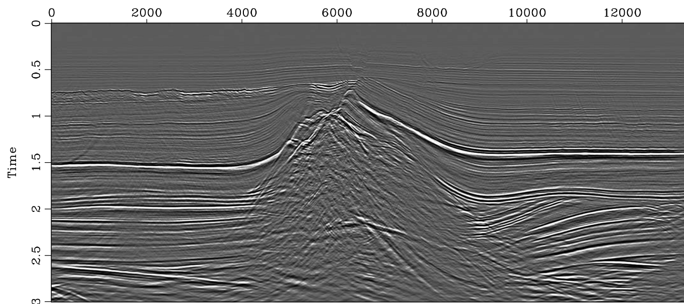
(b) Stolt migration ( v_0 = 2000 m/s)
