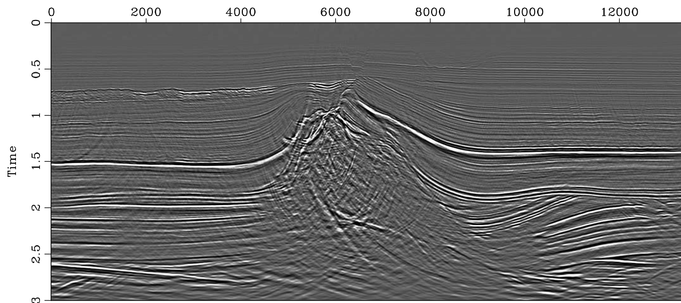
(c) Stolt-stretch migration ( W = 0.5 )
