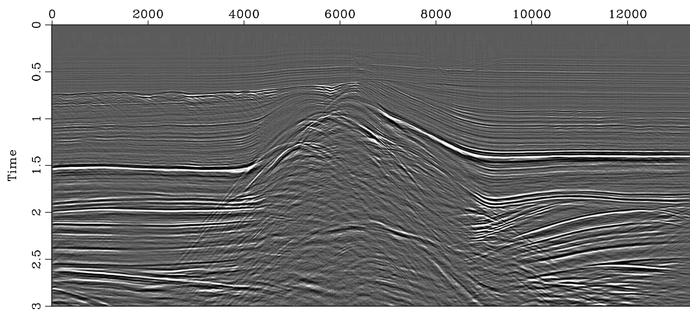
(a) DMO-stack data
