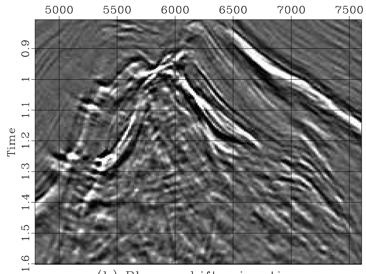
(b) Phase-shift migration
