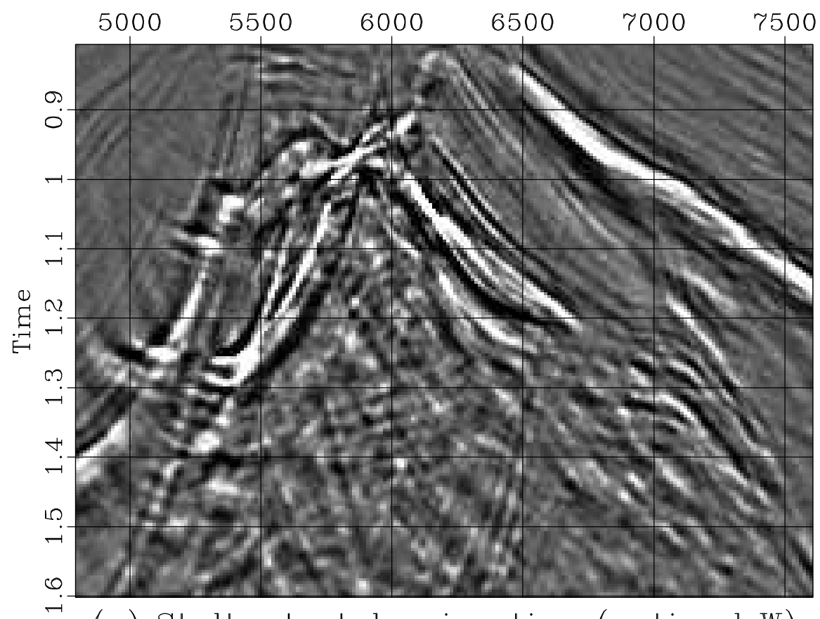
(a) Stolt-stretch migration (optimal W )
