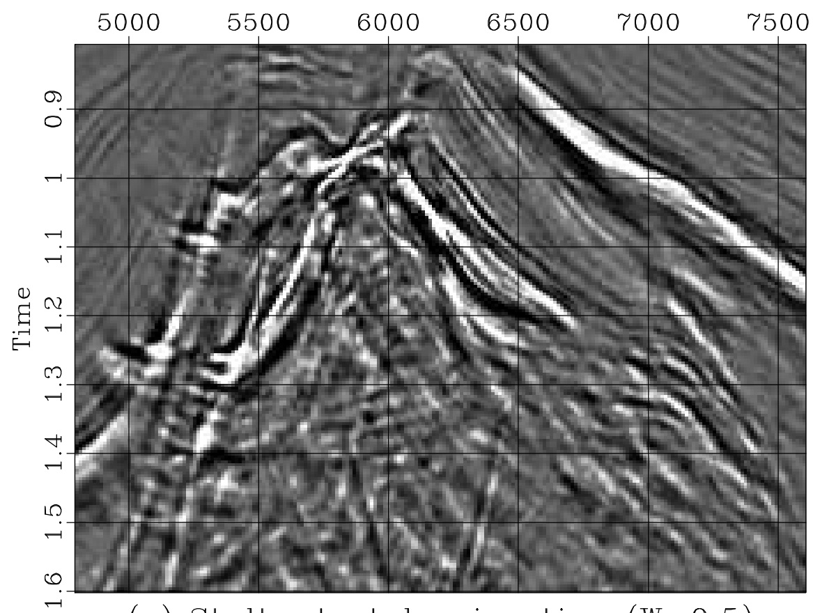
(c) Stolt-stretch migration ( W=0.5 )
