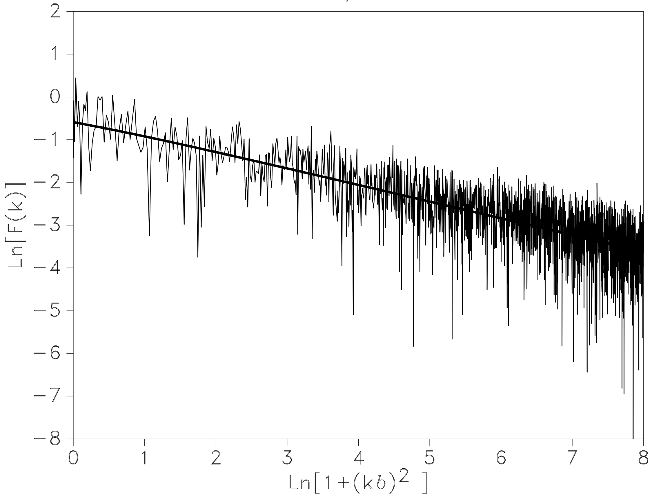
Estimation on synthetic H = 0.25
