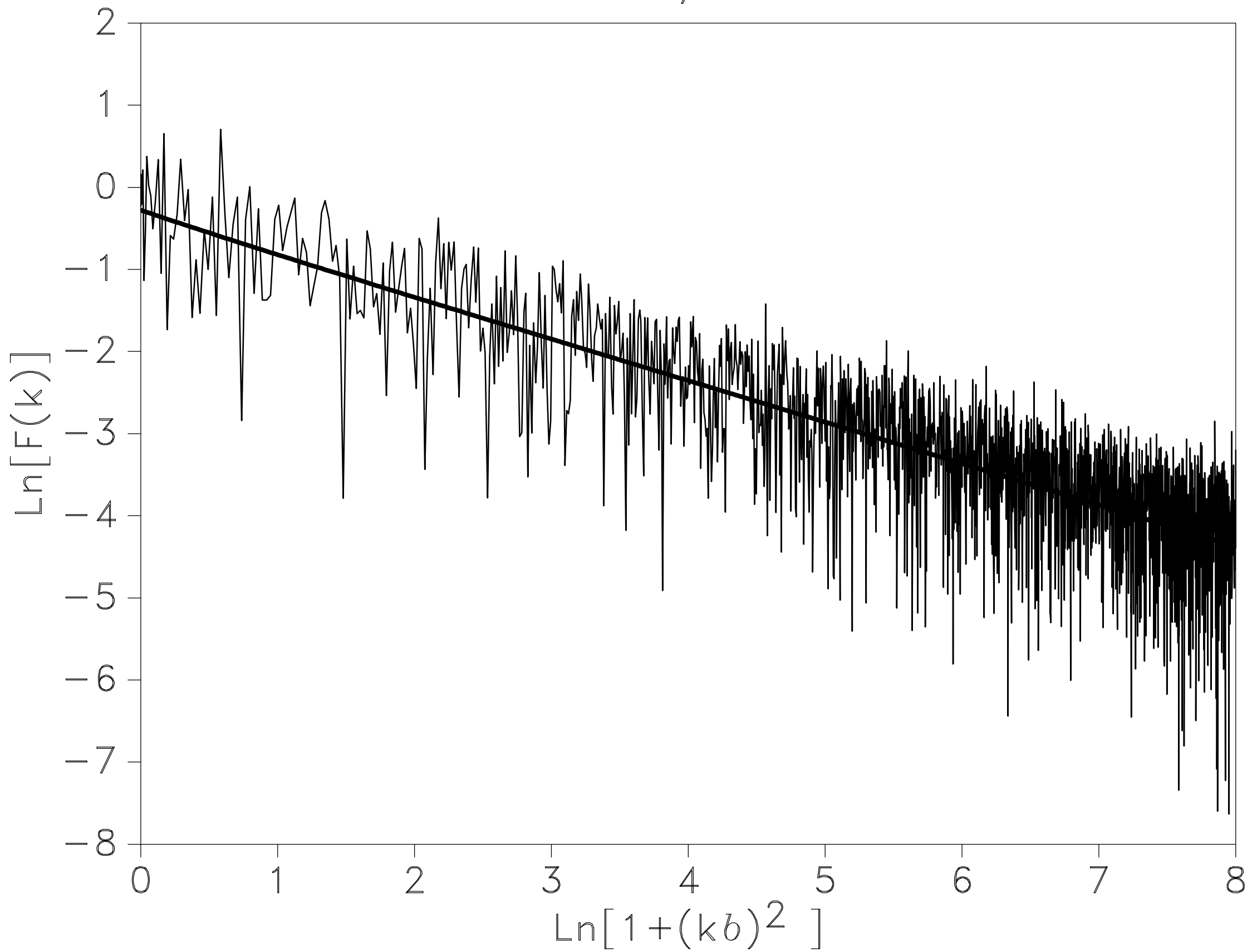
Estimation on synthetic H = 0.5
