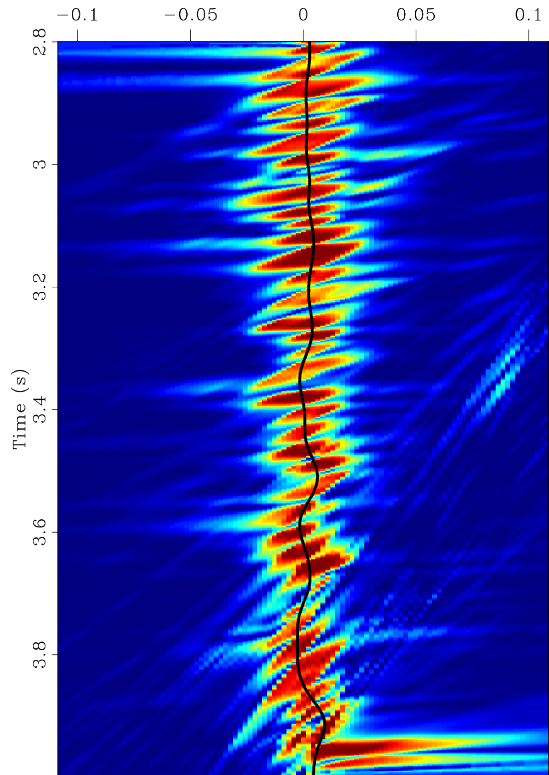
(b) AVO-Friendly Semblance Scan
