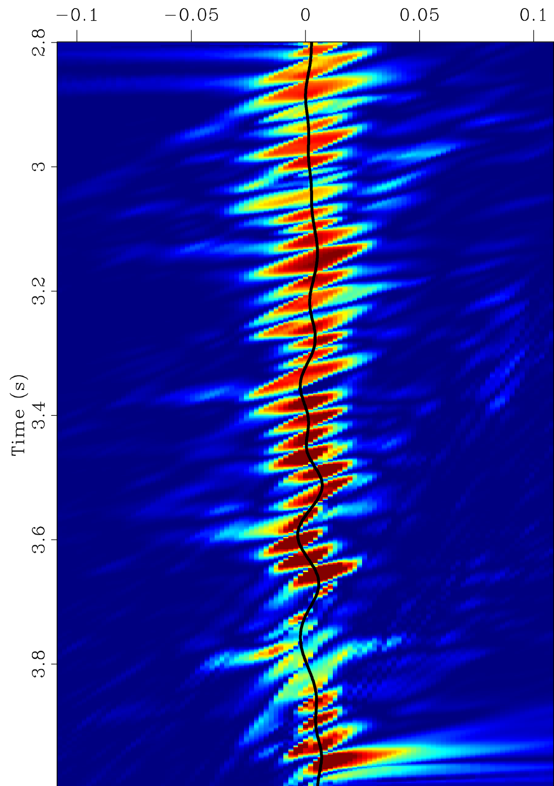
(a) Semblance Scan
