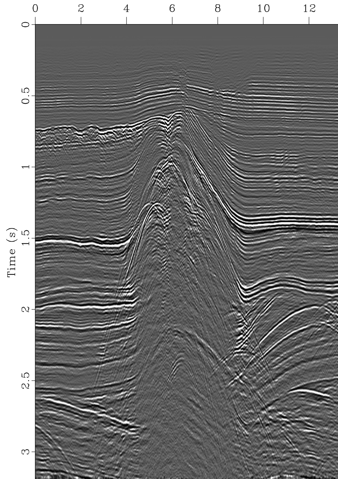
Seislet Stack
